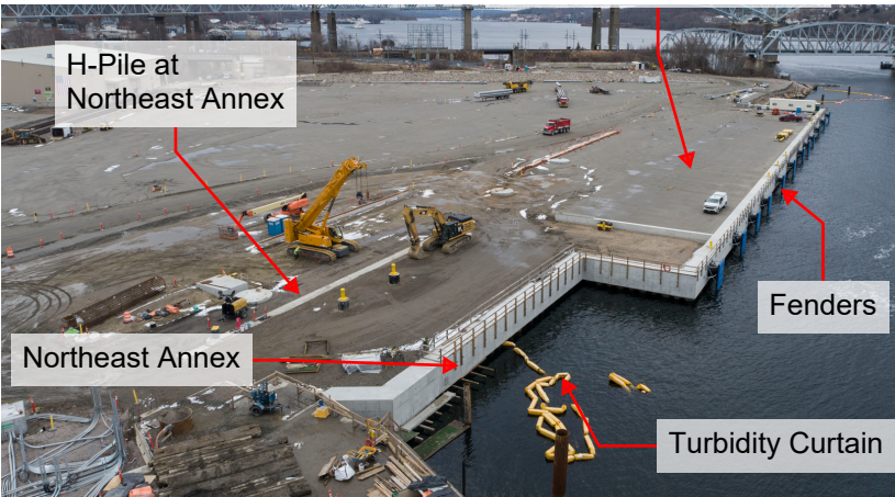
Delivery Berth Heavy Lift Platform
